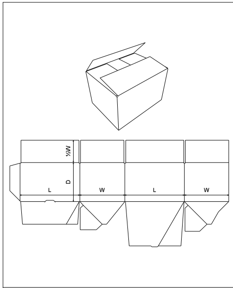
FEFCO\0700 - Ready Glued Cases\ FEFCO 0701
