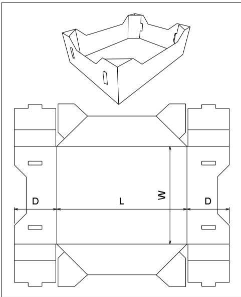
FEFCO\0700 - Ready Glued Cases\ FEFCO 0771
