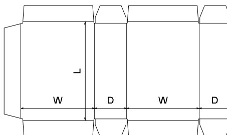
FEFCO\0400 - Folder Type Boxes\ FEFCO 0406
