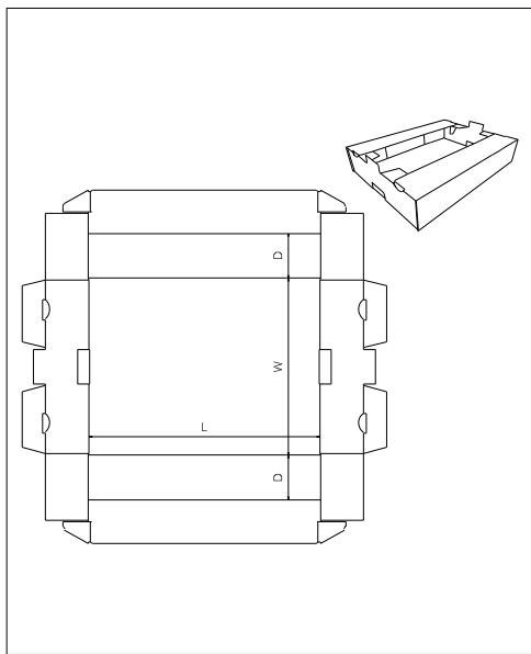
FEFCO\0400 - Folder Type Boxes\ FEFCO 0436
