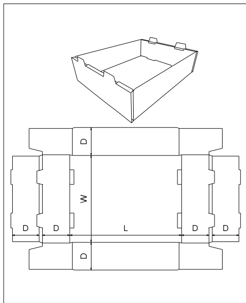
FEFCO\0400 - Folder Type Boxes\ FEFCO 0435
