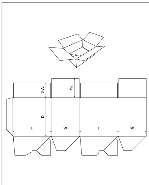
FEFCO\0700 - Ready Glued Cases\ FEFCO 0712
