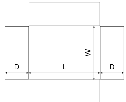
FEFCO\0400 - Folder Type Boxes\ FEFCO 0458
