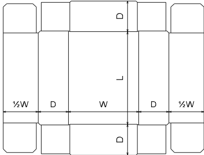
FEFCO\0400 - Folder Type Boxes\ FEFCO 0416
