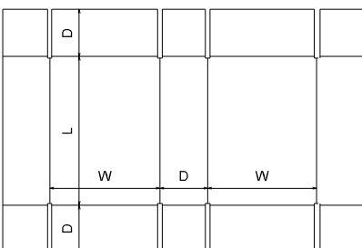
FEFCO\0400 - Folder Type Boxes\ FEFCO 0409
