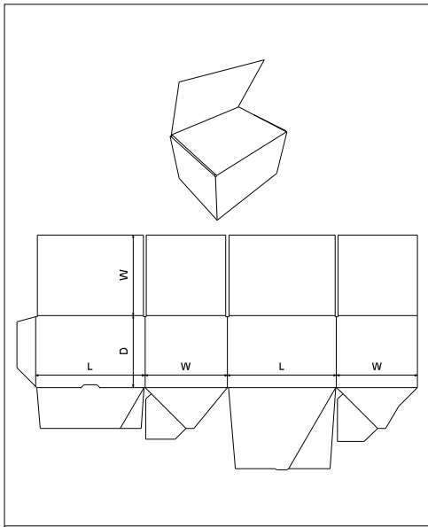
FEFCO\0700 - Ready Glued Cases\ FEFCO 0703
