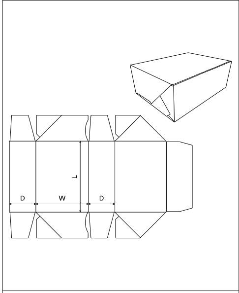
FEFCO\0700 - Ready Glued Cases\ FEFCO 0751
