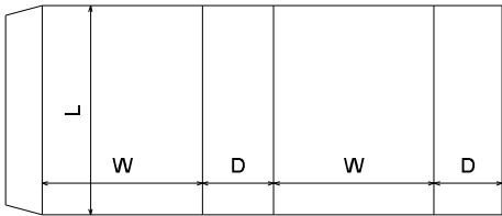
FEFCO\0500 - Slide Type Boxes\ FEFCO 0503
