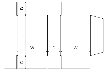
FEFCO\0400 - Folder Type Boxes\ FEFCO 0410
