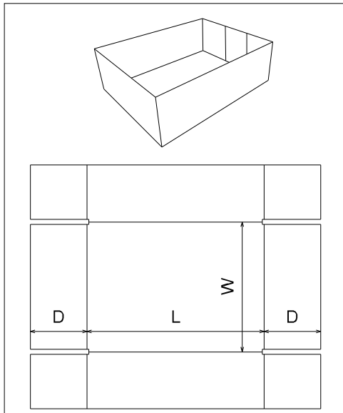
FEFCO\0400 - Folder Type Boxes\ FEFCO 0453
