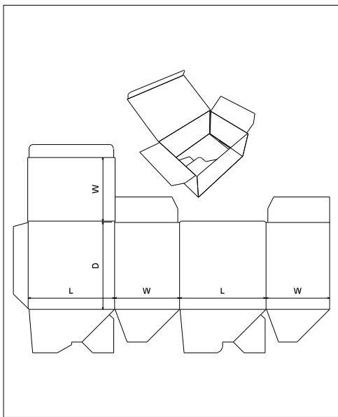
FEFCO\0700 - Ready Glued Cases\ FEFCO 0713
