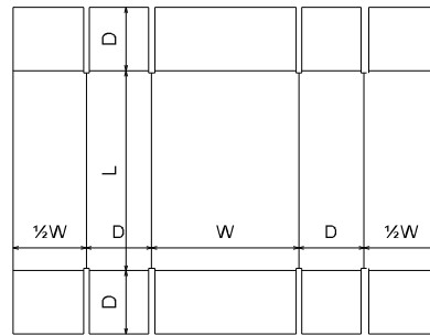
FEFCO\0400 - Folder Type Boxes\ FEFCO 0411
