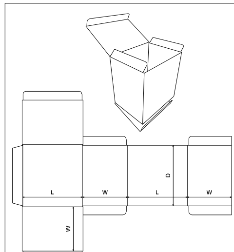
FEFCO\0200 - Slotted Type Boxes\ FEFCO 0210 - Tuck to Front Container
