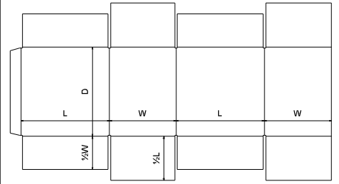
FEFCO\0200 - Slotted Type Boxes\ FEFCO 0204 - All Flaps Meet Slotted Container
