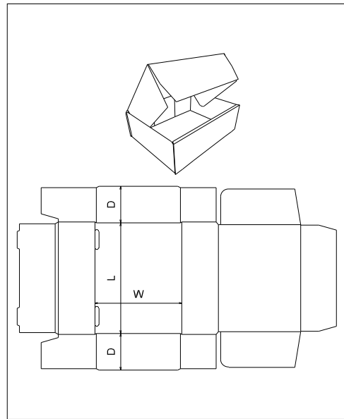
FEFCO\0400 - Folder Type Boxes\ FEFCO 0426
