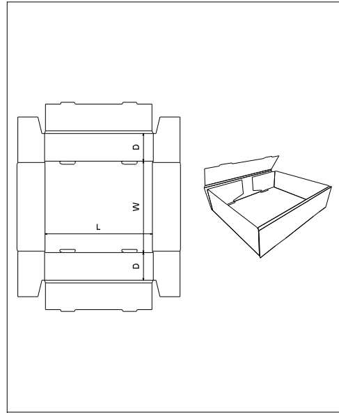
FEFCO\0400 - Folder Type Boxes\ FEFCO 0423
