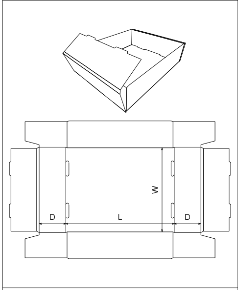
FEFCO\0400 - Folder Type Boxes\ FEFCO 0422
