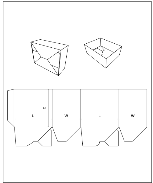
FEFCO\0700 - Ready Glued Cases\ FEFCO 0700
