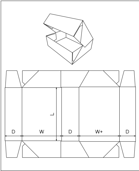
FEFCO\0700 - Ready Glued Cases\ FEFCO 0759
