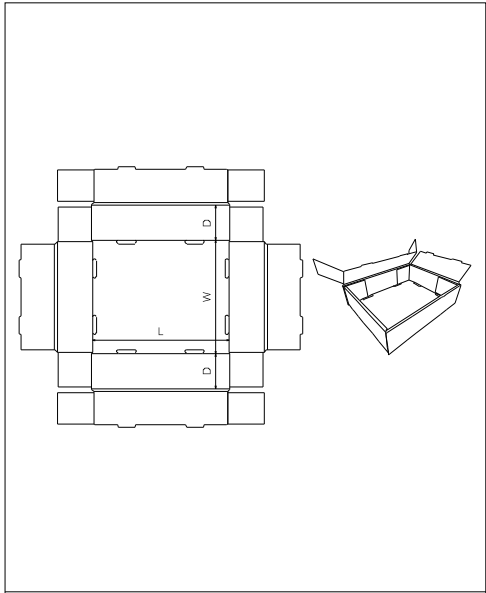
FEFCO\0400 - Folder Type Boxes\ FEFCO 0425
