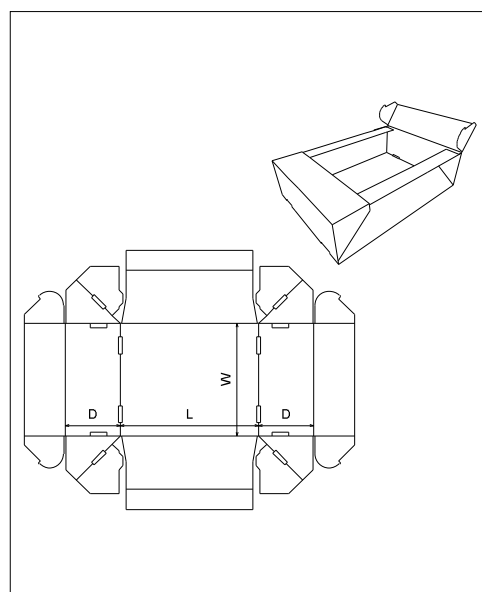
FEFCO\0700 - Ready Glued Cases\ FEFCO 0773
