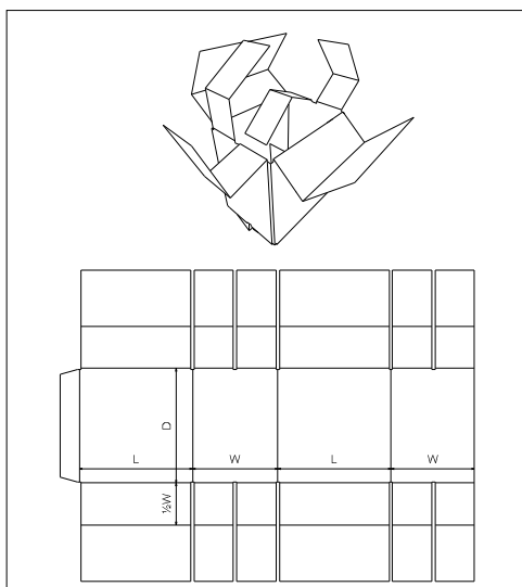
FEFCO\0200 - Slotted Type Boxes\ FEFCO 0208 - Slotted Containers with Holders
