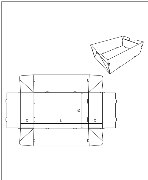
FEFCO\0700 - Ready Glued Cases\ FEFCO 0772
