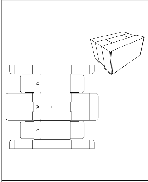
FEFCO\0400 - Folder Type Boxes\ FEFCO 0431
