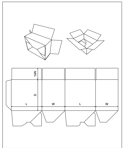
FEFCO\0700 - Ready Glued Cases\ FEFCO 0711
