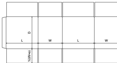
FEFCO\0200 - Slotted Type Boxes\ FEFCO 0202 - Overlapping Slotted Container
