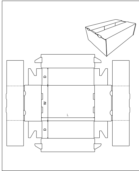
FEFCO\0400 - Folder Type Boxes\ FEFCO 0432
