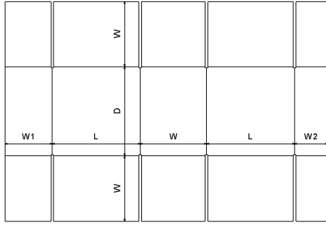
FEFCO\0200 - Slotted Type Boxes\ FEFCO 0231
