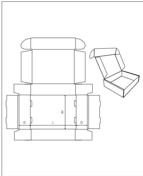
FEFCO\0400 - Folder Type Boxes\ FEFCO 0427
