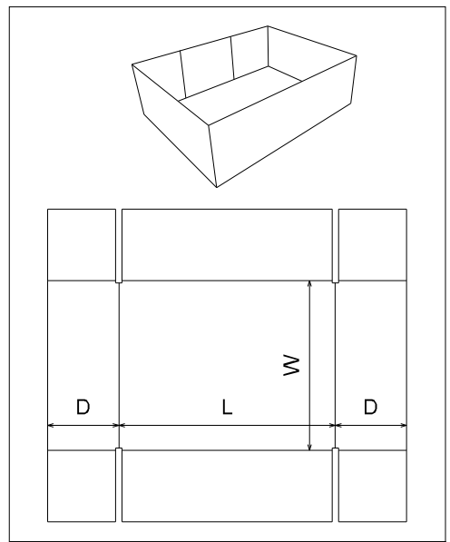
FEFCO\0900 - Interior Fitments\FEFCO 0911
