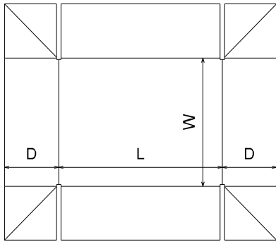
FEFCO\0400 - Folder Type Boxes\ FEFCO 0448
