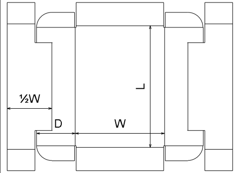
FEFCO\0400 - Folder Type Boxes\ FEFCO 0446
