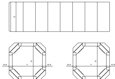
FEFCO\0300 - Telescope Type Box\ FEFCO 0351
