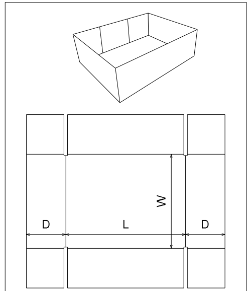
FEFCO\0400 - Folder Type Boxes\ FEFCO 0452
