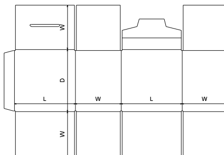
FEFCO\0200 - Slotted Type Boxes\ FEFCO 0218
