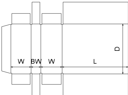
FEFCO\0600 - Rigid Type Boxes\ FEFCO 0621
