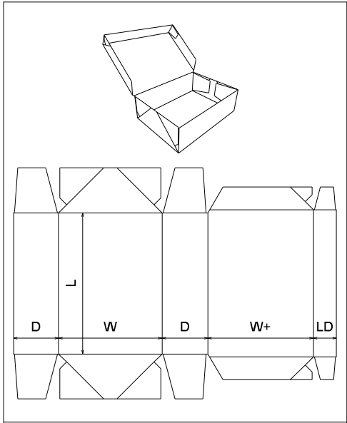
FEFCO\0700 - Ready Glued Cases\ FEFCO 0761
