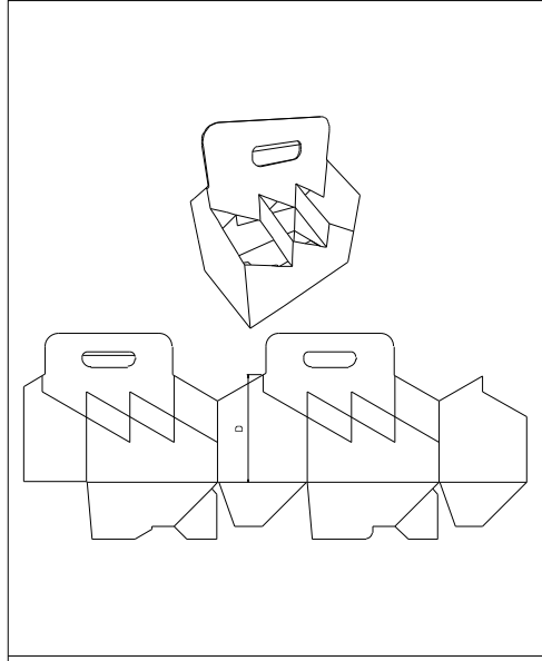
FEFCO\0700 - Ready Glued Cases\ FEFCO 0717 - Bottle Carrier
