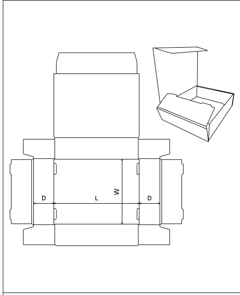
FEFCO\0400 - Folder Type Boxes\ FEFCO 0421
