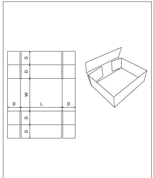
FEFCO\0400 - Folder Type Boxes\ FEFCO 0455
