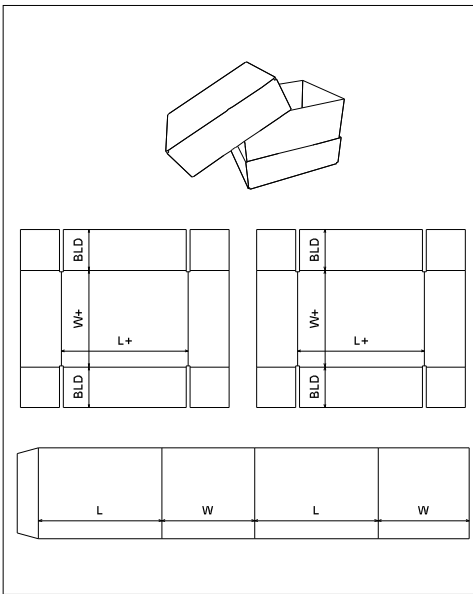
FEFCO\0300 - Telescope Type Box\ FEFCO 0310
