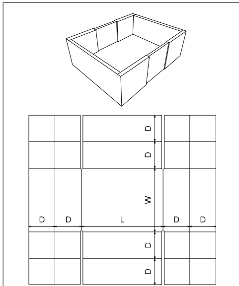
FEFCO\0400 - Folder Type Boxes\ FEFCO 0456
