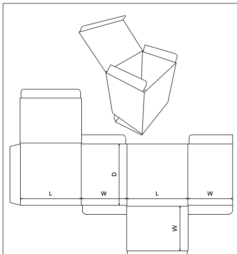
FEFCO\0200 - Slotted Type Boxes\ FEFCO 0211 - Tuck to Front Top, Tuck to Back Base
