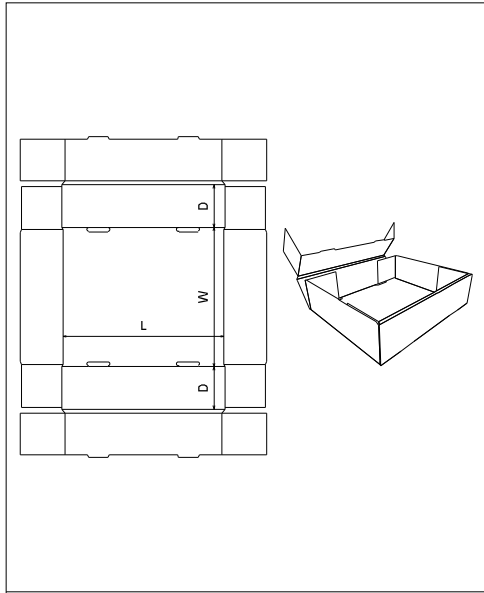
FEFCO\0400 - Folder Type Boxes\ FEFCO 0424
