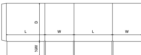
FEFCO\0200 - Slotted Type Boxes\ FEFCO 0200 - Open Slotted Container
