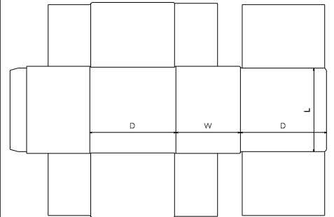
FEFCO\0400 - Folder Type Boxes\ FEFCO 0443
