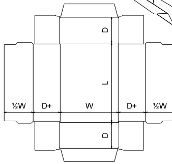
FEFCO\0400 - Folder Type Boxes\ FEFCO 0415
