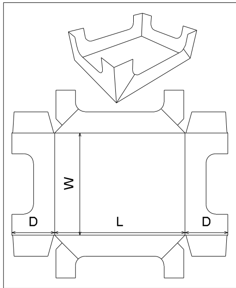
FEFCO\0700 - Ready Glued Cases\ FEFCO 0770
