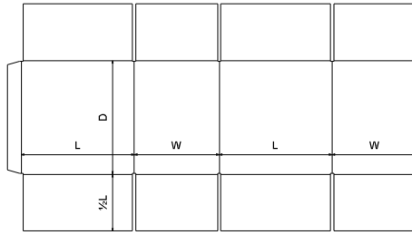
FEFCO\0200 - Slotted Type Boxes\ FEFCO 0205 - Width Panels Meet, Slotted Container
