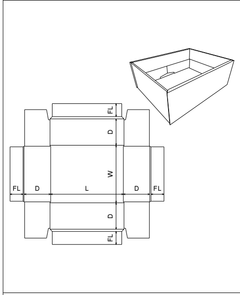
FEFCO\0400 - Folder Type Boxes\ FEFCO 0430
