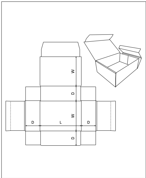
FEFCO\0400 - Folder Type Boxes\ FEFCO 0428
