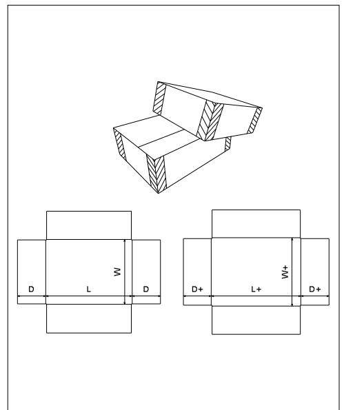
FEFCO\0300 - Telescope Type Box\ FEFCO 0302
