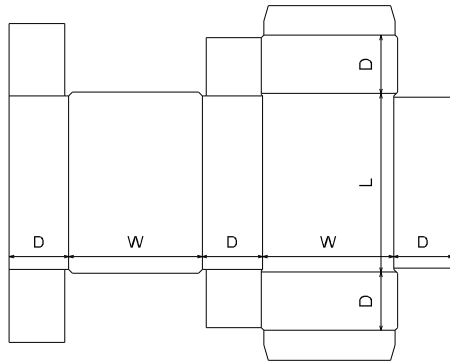
FEFCO\0400 - Folder Type Boxes\ FEFCO 0447
