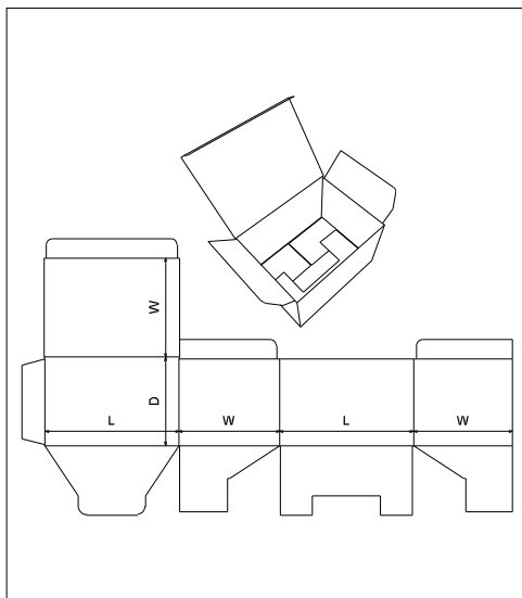
FEFCO\0200 - Slotted Type Boxes\ FEFCO 0215 - Tuck to Front Top, Envelope Base
