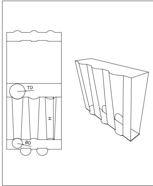
FEFCO\0700 - Ready Glued Cases\ FEFCO 0752 - Glass Pack
