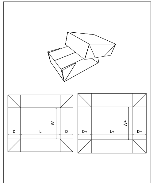
FEFCO\0300 - Telescope Type Box\ FEFCO 0309
