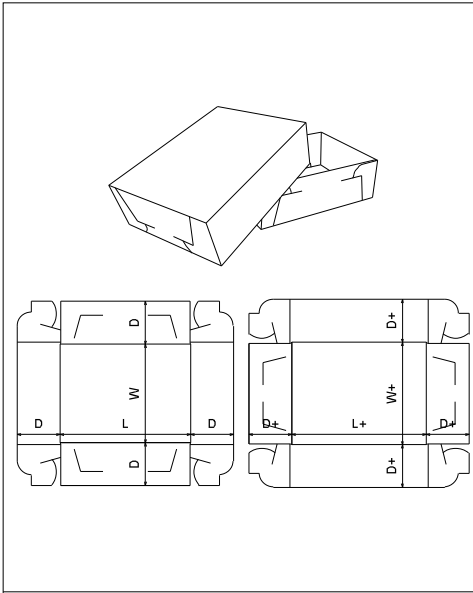
FEFCO\0300 - Telescope Type Box\ FEFCO 0307
