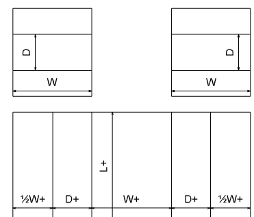
FEFCO\0400 - Folder Type Boxes\ FEFCO 0405
