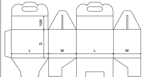
FEFCO\0200 - Slotted Type Boxes\ FEFCO 0217 - Carry Handle Top, Envelope Base
