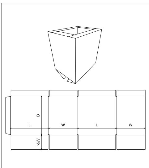
FEFCO\0200 - Slotted Type Boxes\ FEFCO 0209 - Flange Top, Regular Slotted Base
