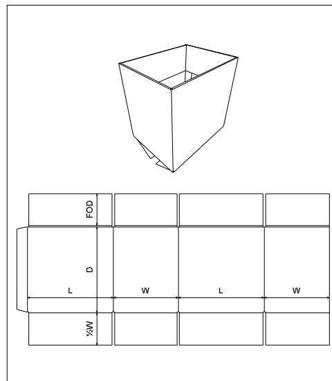
FEFCO\0200 - Slotted Type Boxes\ FEFCO 0214 - Roll Over Top Slotted Container
