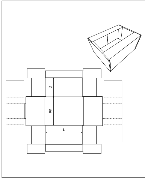
FEFCO\0400 - Folder Type Boxes\ FEFCO 0433
