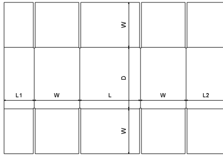
FEFCO\0200 - Slotted Type Boxes\ FEFCO 0230
