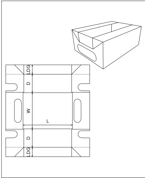
FEFCO\0400 - Folder Type Boxes\ FEFCO 0434
