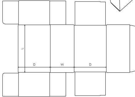
FEFCO\0400 - Folder Type Boxes\ FEFCO 0444
