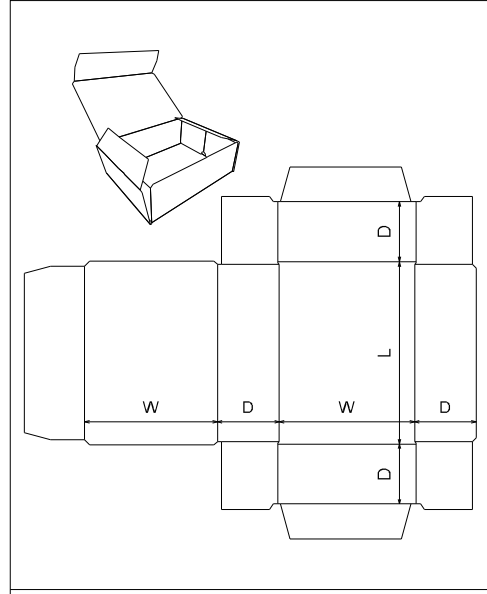
FEFCO\0400 - Folder Type Boxes\ FEFCO 0420
