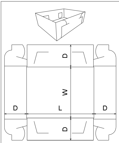
FEFCO\0400 - Folder Type Boxes\ FEFCO 0457
