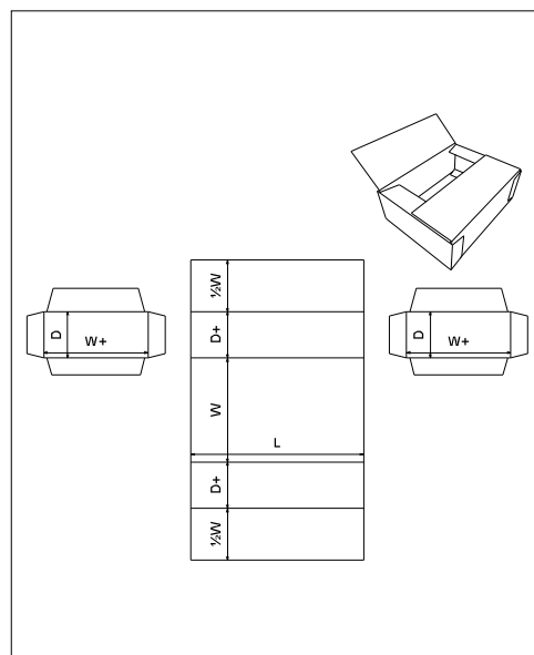
FEFCO\0600 - Rigid Type Boxes\ FEFCO 0605
