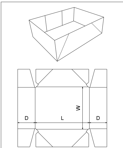
FEFCO\0400 - Folder Type Boxes\ FEFCO 0451
