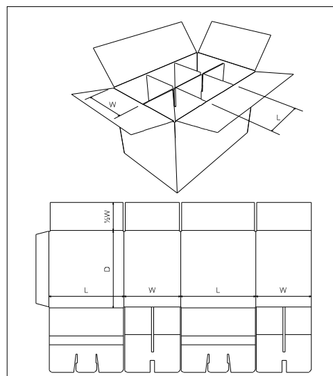
FEFCO\0200 - Slotted Type Boxes\ FEFCO 0207 - Slotted Container with Dividers
