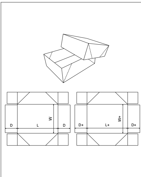
FEFCO\0300 - Telescope Type Box\ FEFCO 0303
