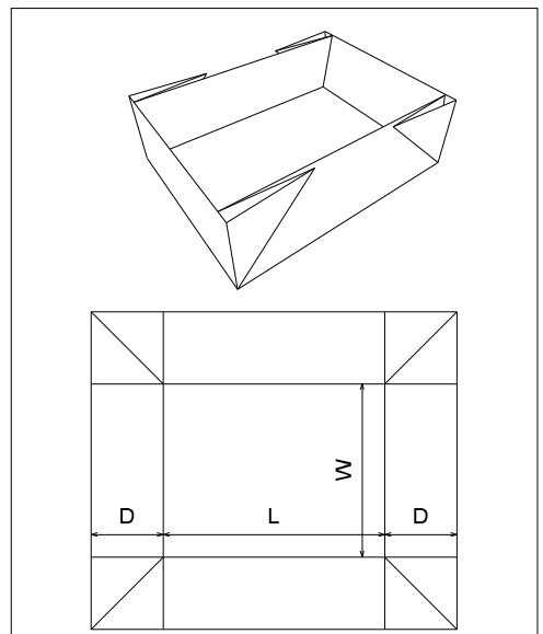
FEFCO\0400 - Folder Type Boxes\ FEFCO 0449
