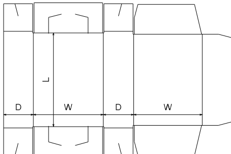
FEFCO\0400 - Folder Type Boxes\ FEFCO 0442
