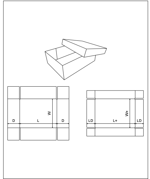
FEFCO\0300 - Telescope Type Box\ FEFCO 0306
