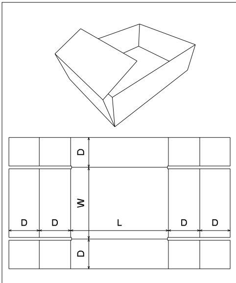
FEFCO\0400 - Folder Type Boxes\ FEFCO 0454
