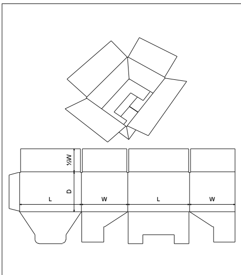
FEFCO\0200 - Slotted Type Boxes\ FEFCO 0216 - Regular Slotted Top, Envelope Base
