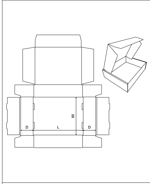
FEFCO\0400 - Folder Type Boxes\ FEFCO 0429
