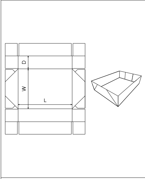
FEFCO\0700 - Ready Glued Cases\ FEFCO 0718
