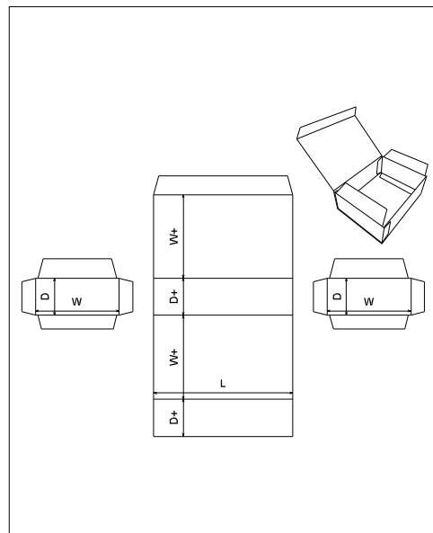
FEFCO\0600 - Rigid Type Boxes\ FEFCO 0608
