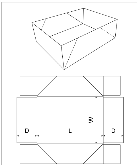
FEFCO\0400 - Folder Type Boxes\ FEFCO 0450
